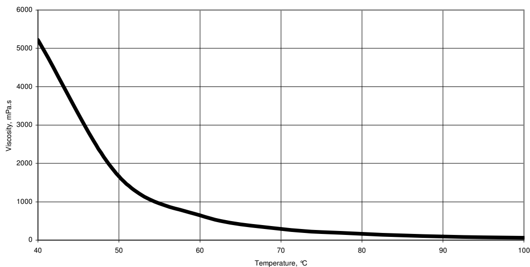
SYLVATAC ® RE5S - Temperature Viscosity Profile
